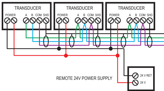
TYPICAL CONNECTION OF MRS-485
