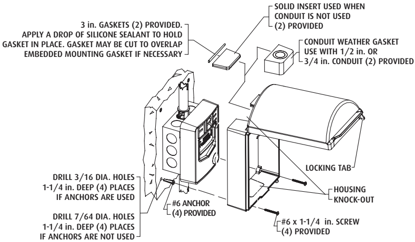
Fig. 4 - SURFACE MOUNTING OPTION
